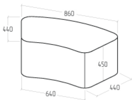
EV-AR-PF-9 860/640x440x450
