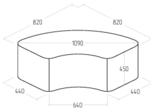
EV-AR-PF-10 1090/640x440x450
