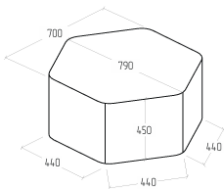
EV-AR-PF-7 790/700x440x450
