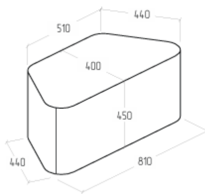
EV-AR-PF-8 810/510x440x450
